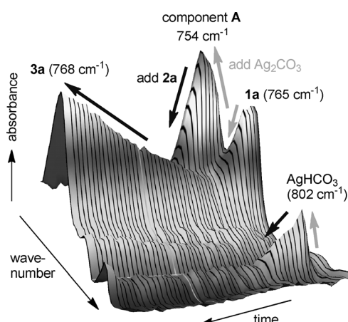
Figure 1. Profile of the stepwise stoichiometric reaction between 1a , Ag 2 CO 3 , and 2a in DMSO at 80 °C monitored by in situ IR spectroscopy.
